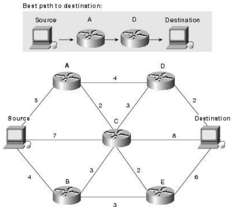
Figure: The DRP Determines the Optimal Route Through a DECnet Phase IV Network
